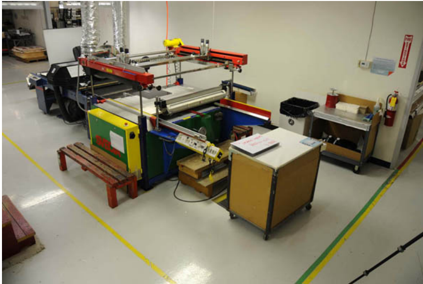
1 Color Svecia 3/4 Automatic Screen Printing Press 32 x 42 MSI has 3 identical presses this style
